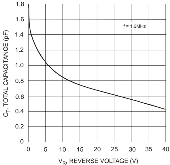
Fig. 3 Typical Capacitance
